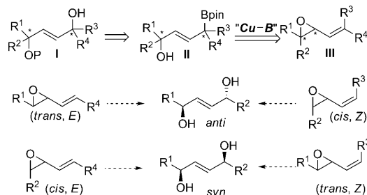
Scheme 1. Proposed diastereoselective synthesis of 1,4-diols. pin = pinacolato.
